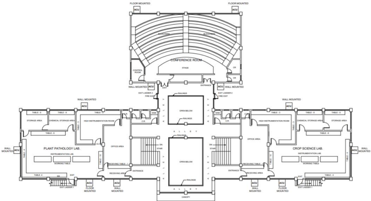
SECOND FLOOR PLAN SCALE 1 : 150m.
