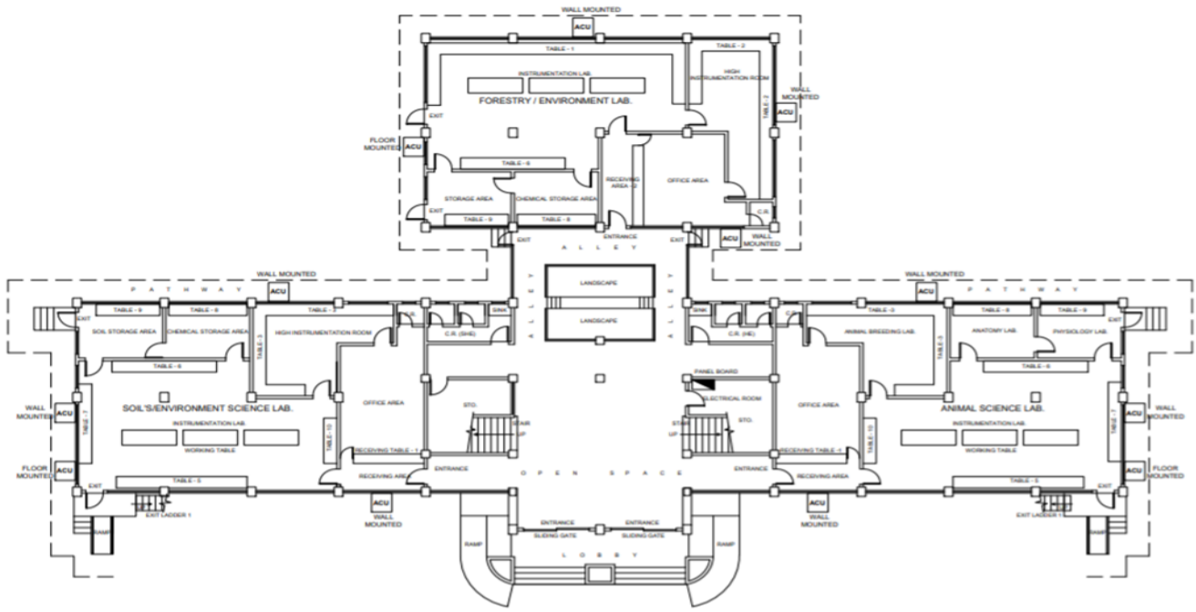
GROUND FLOOR PLAN SCALE 1 : 150m.
